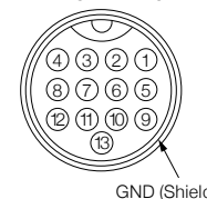
Connector <Pin Assignment Figure>
